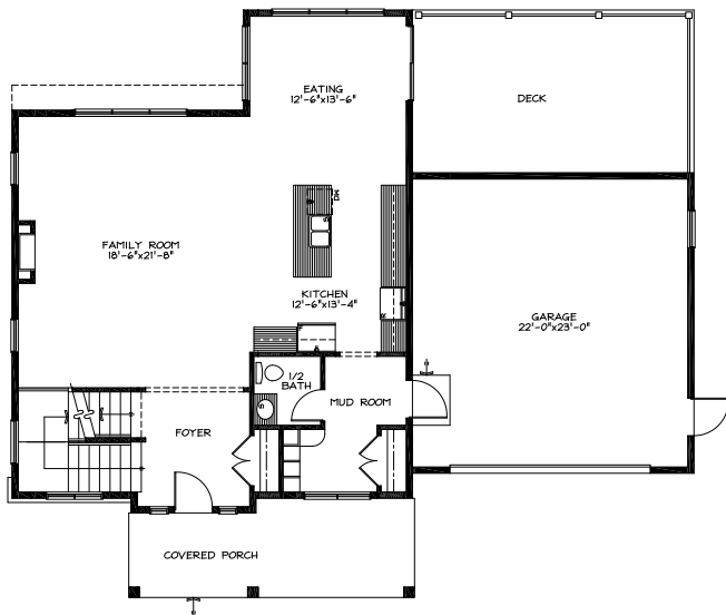
TWO STOREY - MAIN FLOOR 1,099.99 SQ FT
