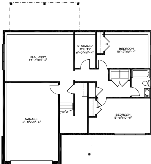
SPLIT ENTRY - LOWER FLOOR 948.58 SQFT
