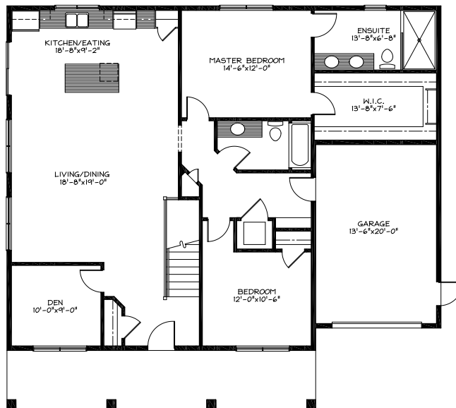
BUNGALOW OPTION 2 - MAIN FLOOR 1,545.24 SQFT
