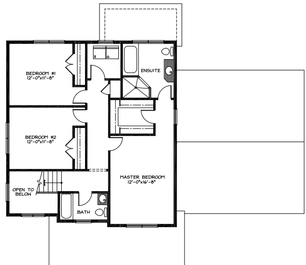
TWO STOREY - SECOND FLOOR 1,008.40 SQ FT
