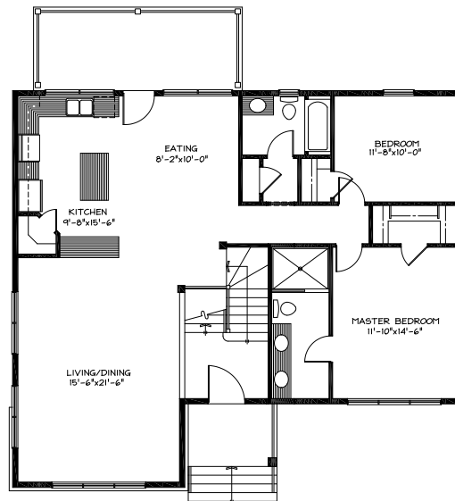
SPLIT ENTRY - UPPER FLOOR 1,334.00 SQFT
