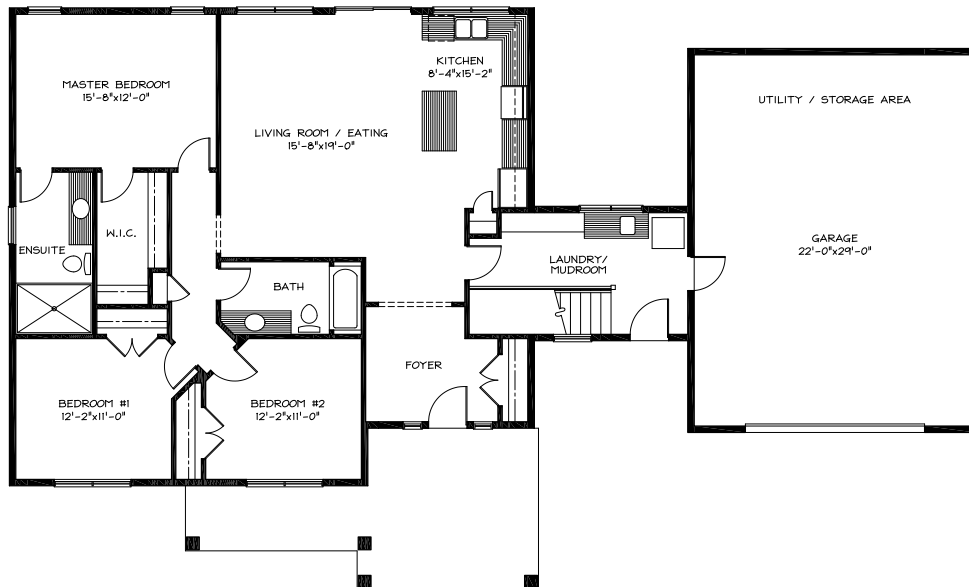
BUNGALOW OPTION I - MAIN FLOOR 1,598.16 SQFT
